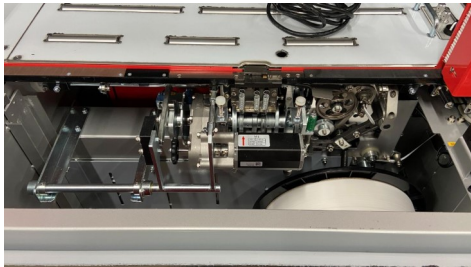
Robust & Compact Mechanical Strapping Head
